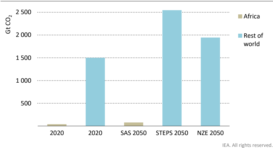
Figure 4.2 ▶ Global cumulative energy-related CO 2 emissions and African share since 1890 by scenario
